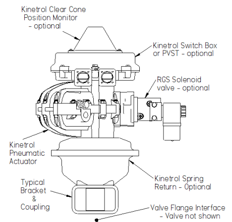
Figure 1 Typical Kinetrol Actuator Arrangement
